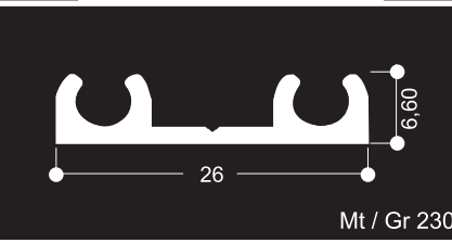
8024 - Alt Ray / Bottom Rail
