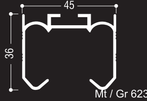
8018 B - Alt Ray / Bottom Rail
