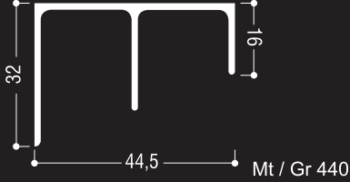
8018 A - Alt Ray / Bottom Rail
